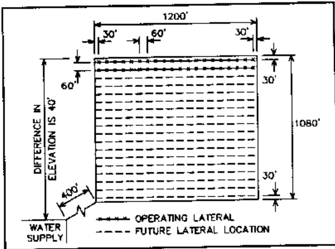
Figure 1. Schematic of a portable hand-move aluminum pipe irrigation system.
